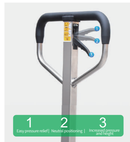
Lightweight upgraded rubber-coated handle Manual pressure release + foot-operated pressure release
